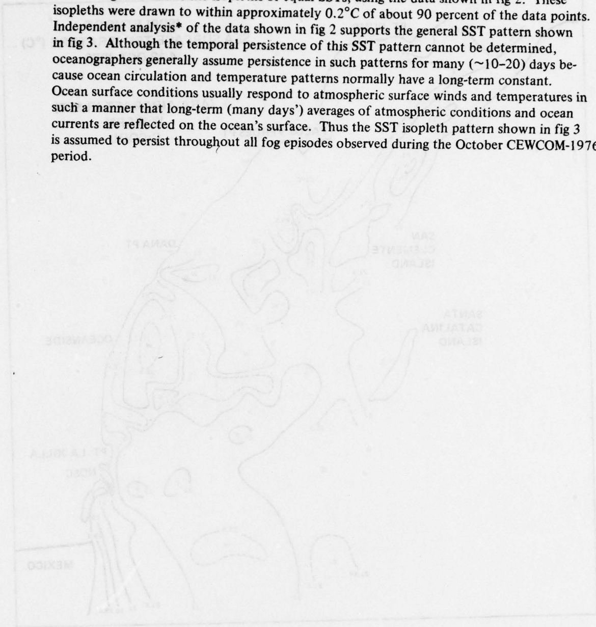
Figure 3 - Isopleths of equal surface temperature according to the data in fig 2.
